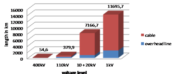
Figure 2: Overview line/cable length of Wiener Netze GmbH (as of 2014, [5])
