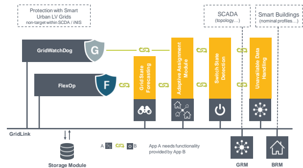
Figure 1: Set of applications supporting a Plug & Automate approach within an intelligent secondary substation
