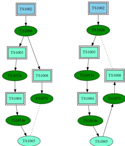
Figure 6: A valid (left) and an invalid topology (right)
