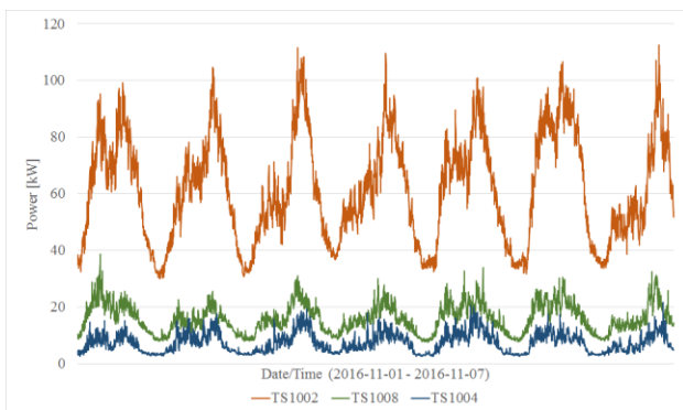
Figure 7: Power profiles of three grid monitoring devices
