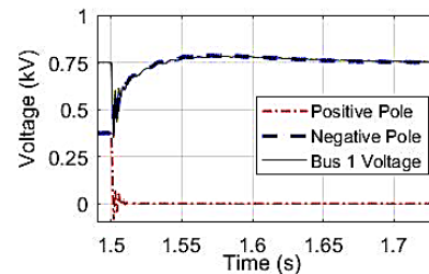
Fig. 9. Bus 1 voltage with overcurrent protection during the location 1 P-G fault condition.
