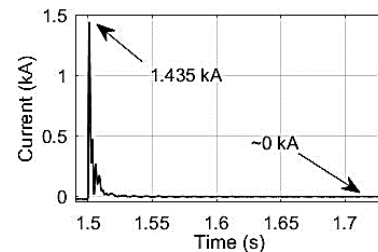
Fig. 8. Fault current measured at D1 with overcurrent protection during the location 1 positive P-G fault condition.
