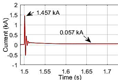
Fig. 7. Fault current measured at D2 with overcurrent protection during the location 1 P-P fault condition.
