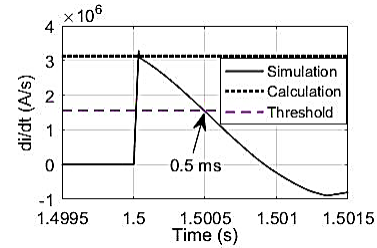
Fig. 13. Measured and calculated di/dt in the D1 side when P-P fault happens in location 1.
