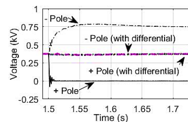
Fig. 11. Bus 1 voltage with differential protection during the location 1 P-G fault condition.
