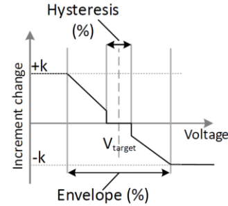
Figure 5: Voltage trigger points for increment of injected and absorbed power for AIMD voltage support algorithm.
