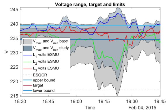
Figure 9: Comparison of phase-to-neutral voltage range on the feeder for baseline and with AIMD.
