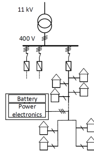
Figure 2: Diagram of a typical ESMU location on low a voltage feeder.
