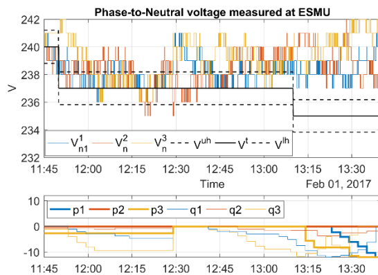
Figure 13: (Top) Profile of phase-to-neutral voltages measured at the ESMU during the trial, with overlaid target voltage and hysteresis band. (Bottom) ESMU kW and kVAr instructions during trial.
