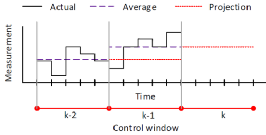
Figure 4: Approximation of measurements through projection of average
