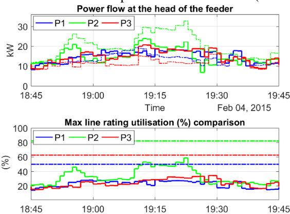
Figure 7: Top - active power measures at the head of the feeder per phase: (-) with ESMU, (--) baseline; Bottom - Line utilisation per phase: (-) ESMU, (--) maximum line utilisation in baseline study.
