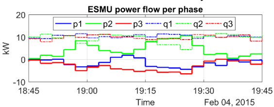
Figure 8: Active and reactive instructions per phase for ESMU performing phase balancing and PF correction during evening peak demand. Positive values indicate power injected into the network.
