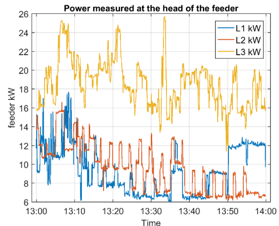
Figure 3: Example of demand variability at 5-second resolution on a LV feeder
