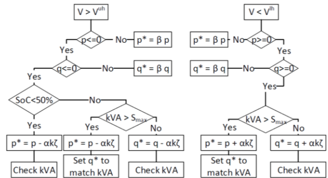
Figure 6: AIMD decision tree for (left) high voltage events V^{uh} , and (right) low voltage events V^{lh} .
