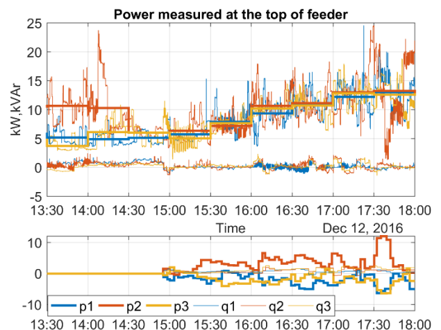
Figure 11: Top – kW (5 second and half-hourly averages) and kVAr profiles measured at top of feeder; Bottom – ESMU kW and kVAr instructions per phase.
