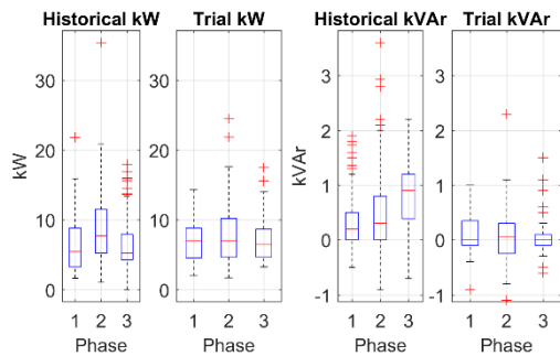
Figure 12: Box plots of half-hourly kW and kVAr per phase from phase-balancing trial and historical data.
