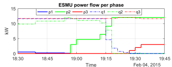
Figure 10: ESMU reactive (--) and active power (-) injection per phase under AIMD voltage support.
