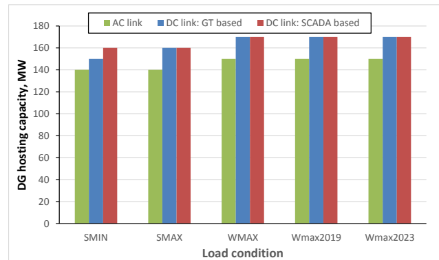
Figure 6. Anglesey network's DG hosting capacity
