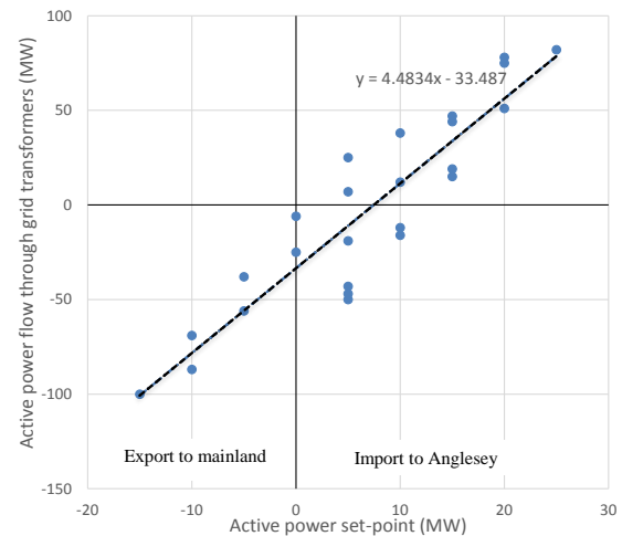
Figure 4. Operation curve for active power set-points using the GT data based control
