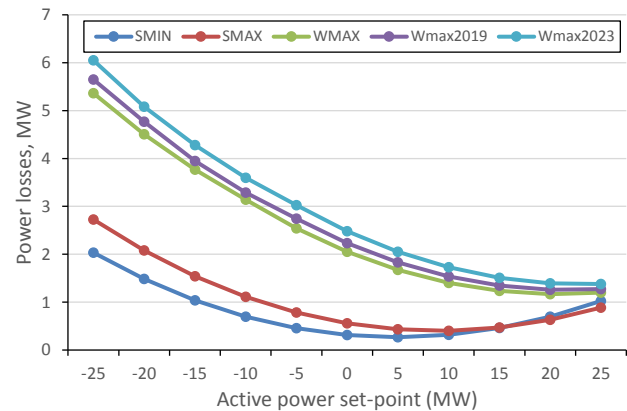
Figure 3. Anglesey network power losses at 0 MW DG
