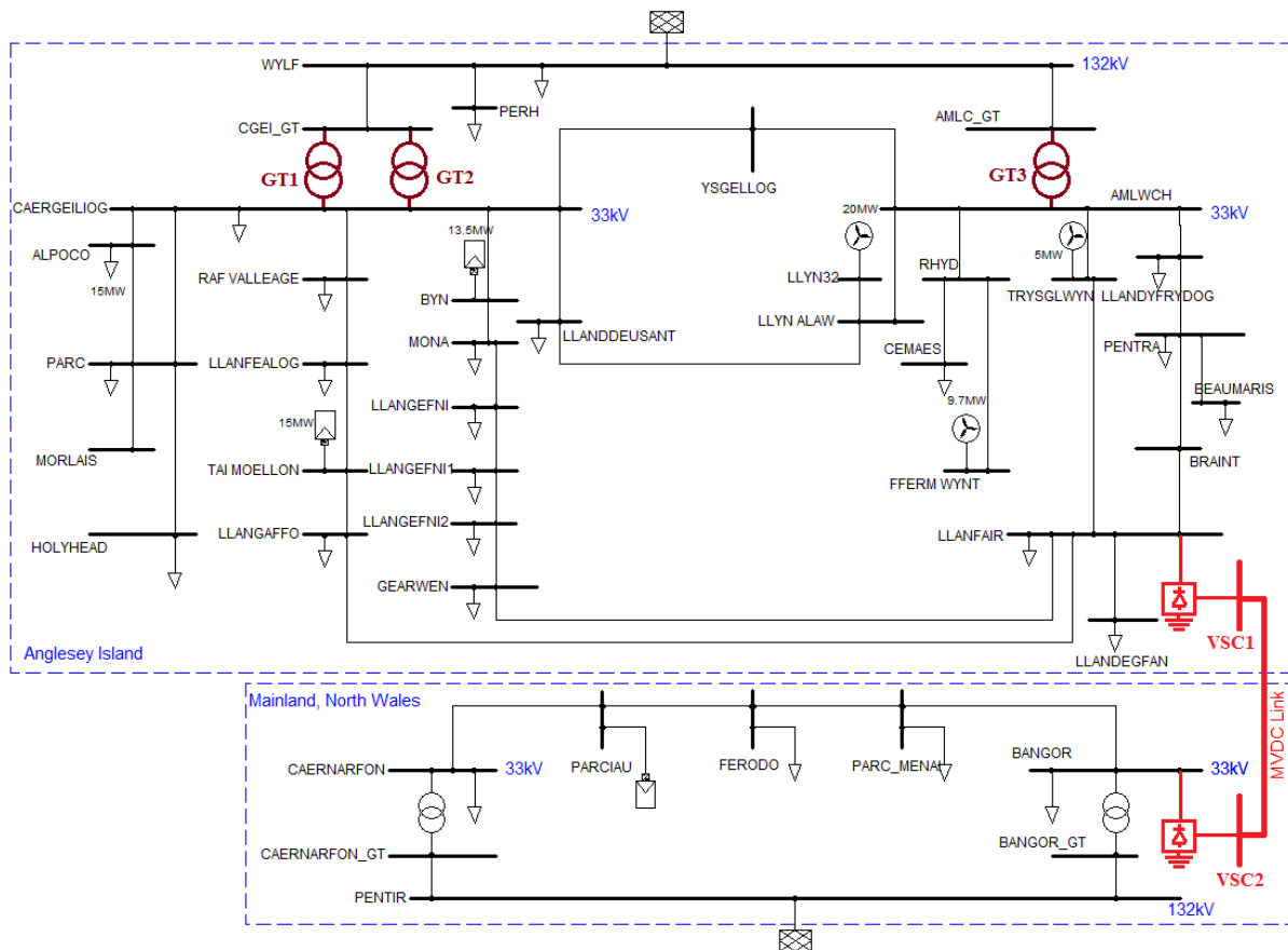
Figure 2. 33 kV network circuit on Anglesey, UK
